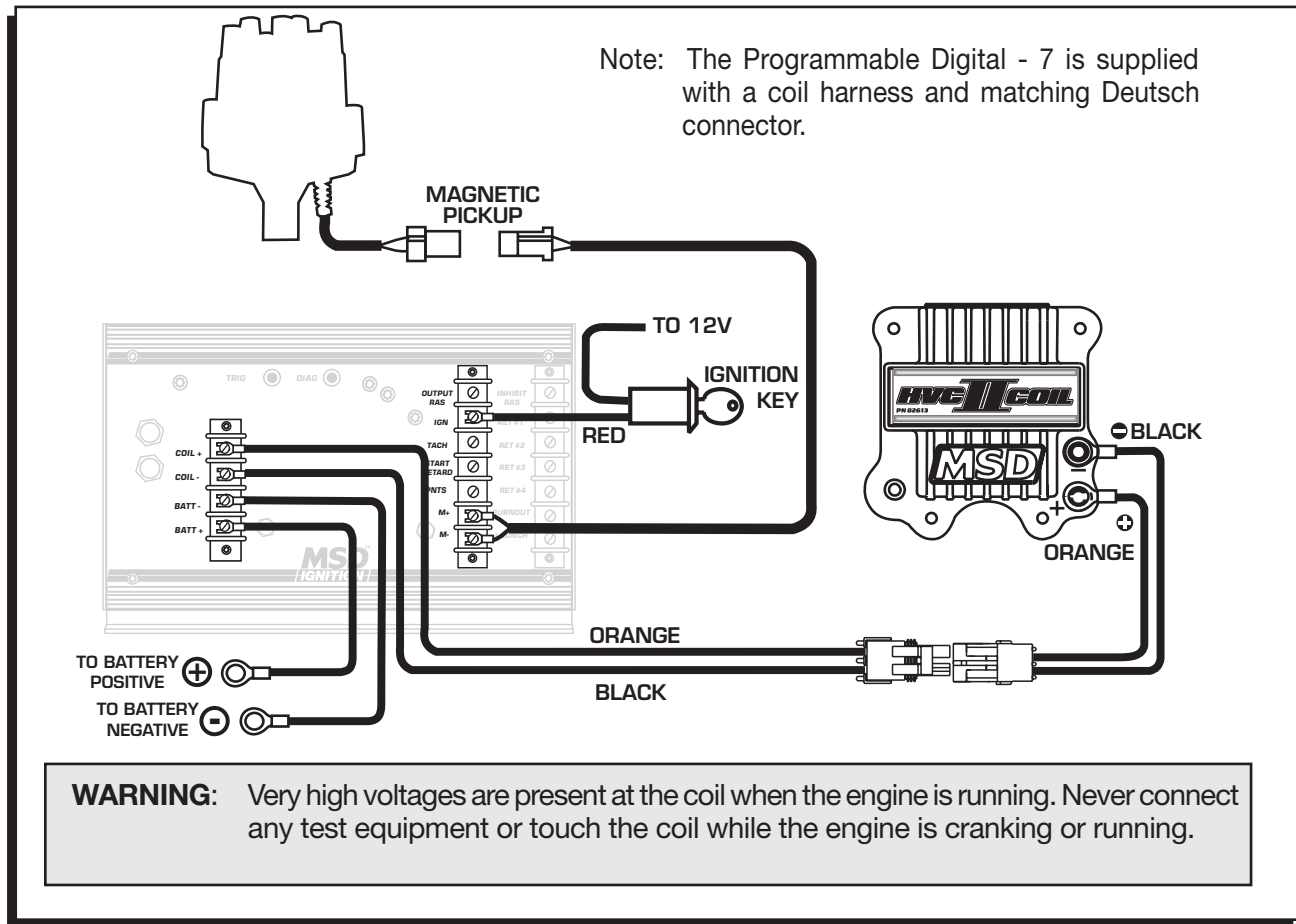
Wiring to an MSD 7AL-3
